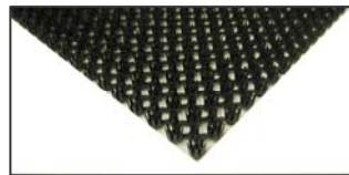
Graphite
